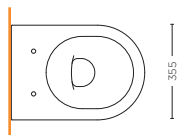
VASO SOSPESO 50R WALL HUNG WC 50R SMMX.S20.W02
