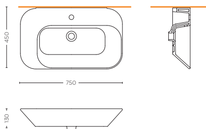
LAVABO LF 75 cm WASHBASIN LF 75 cm SMMX.S10.03
