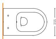
VASO FILO MURO 56R BACK TO WALL WC 56R SMMX.S20.FU04
