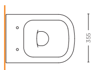
VASO SOSPESO 50Q WALL HUNG WC 50Q SMMX.S20.W01
