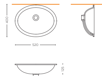
LAVABO DA INCASSO OVALE 52 cm OVAL COUNTERTOP WASHBASIN 52 cm SMMX.S11.22
