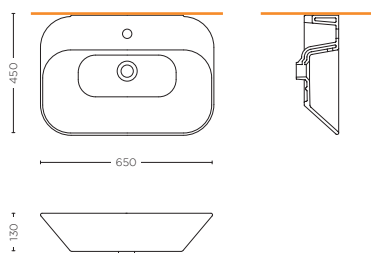
LAVABO 65 cm WASHBASIN 65 cm SMMX.S10.01
