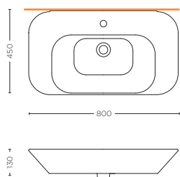
LAVABO 80 cm WASHBASIN 80 cm SMMX.S10.02
