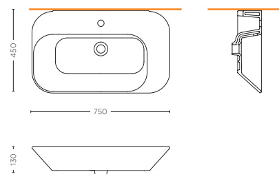
LAVABO RT 75 cm WASHBASIN RT 75 cm SMMX.S10.04
