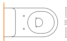
VASO MONOBLOCCO CON CASSETTA 66Q CLOSE COUPLED WC WITH CISTERN 66Q SMMX.S20.CU02 / SMMX.S28.01
