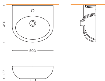
LAVABO 50 cm WASHBASIN 50 cm SDBD.S10.01
