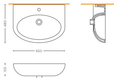
LAVABO 65 cm WASHBASIN 65 cm SDBD.S10.04
