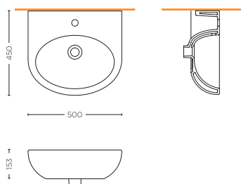
LAVABO 50 cm WASHBASIN 50 cm SDBD.S10.01
