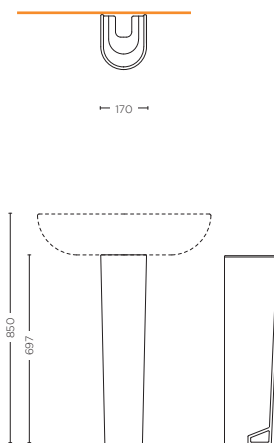
COLONNA PEDESTAL SDBD.S19.F01
