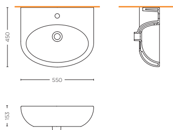
LAVABO 55 cm WASHBASIN 55 cm SDBD.S10.02
