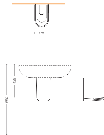
SEMICOLONNA HALF PEDESTAL SDBD.S19.H01
