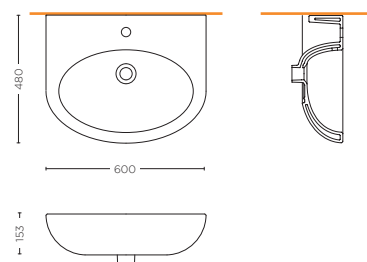
LAVABO 60 cm WASHBASIN 60 cm SDBD.S10.03
