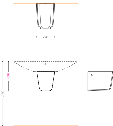
SEMICOLONNA HALF PEDESTAL SCLB.S19.H01
