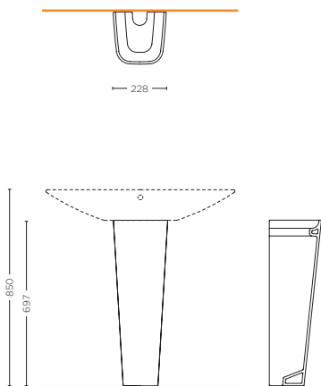
COLONNA PEDESTAL SCLB.S19.F01
