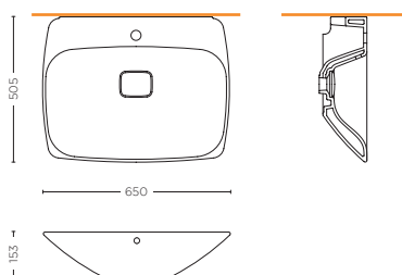
LAVABO 65 cm WASHBASIN 65 cm SCLB.S10.01
