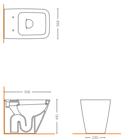
VASO FILO MURO BACK TO WALL WC SCLB.S20.FU01
