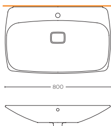
LAVABO 80 cm WASHBASIN 80 cm SCLB.S10.02
